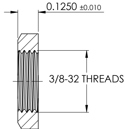
SECTION Y-Y
